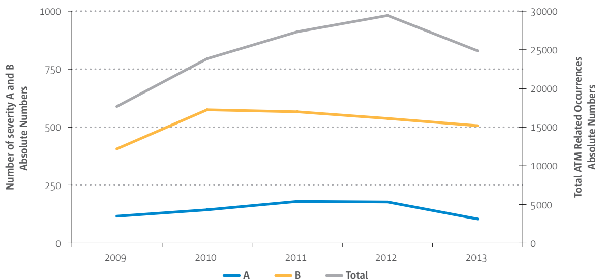
► Figure 53: ATM-related Incidents by Severity A and B (Number of occurrences in absolute numbers)
