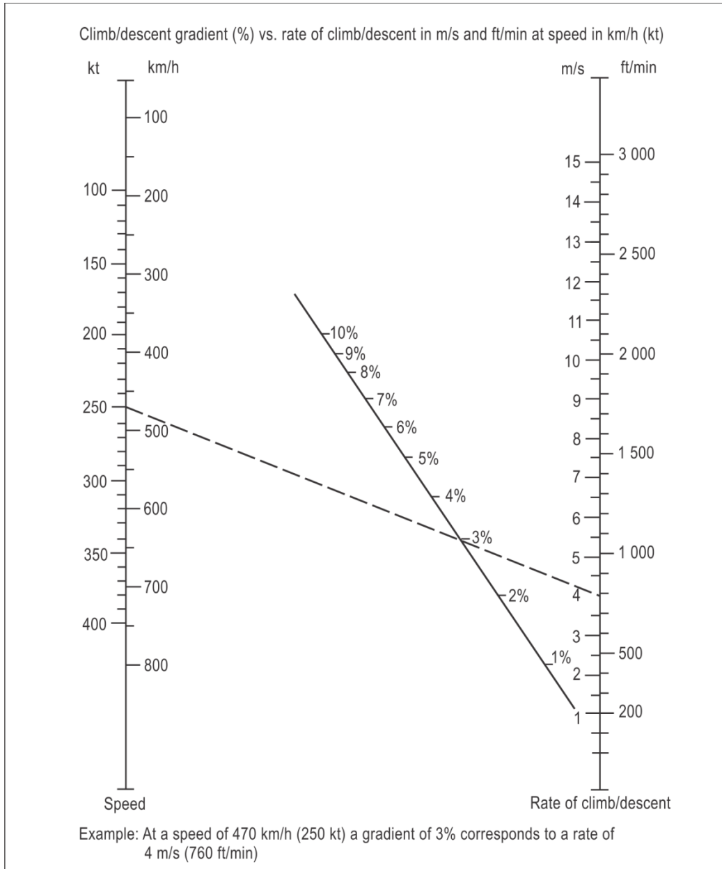
Figure II-2-1-2. Conversion nomogram
