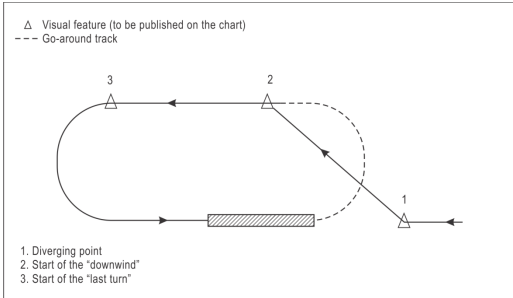
Figure II-5-6-3. Standard track general case
